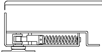
7811 Mechanism
