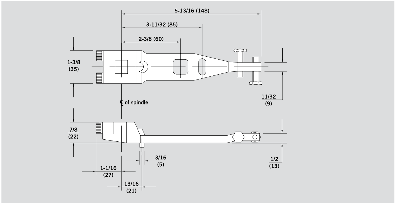
No. 8836S — End load arm specifically designed for tempered glass doors with a short top rail (patch fitting). Requires a minimum \frac{7}{8} " top door rail channel depth.
