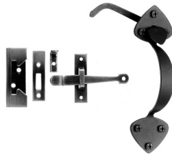
AT4BR: Reverse bevel/closet door. (handle on room side or exterior of storm door) 7-3/4" x 2" proj. 1-5/8"
